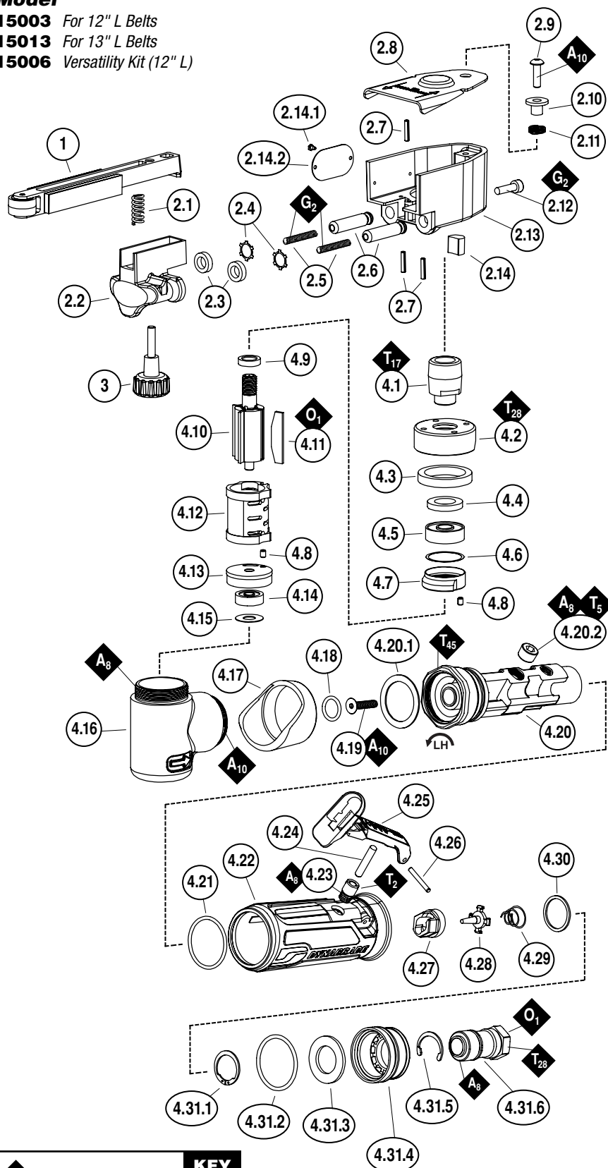
Figure 1 - Versatility Kit (15006)
