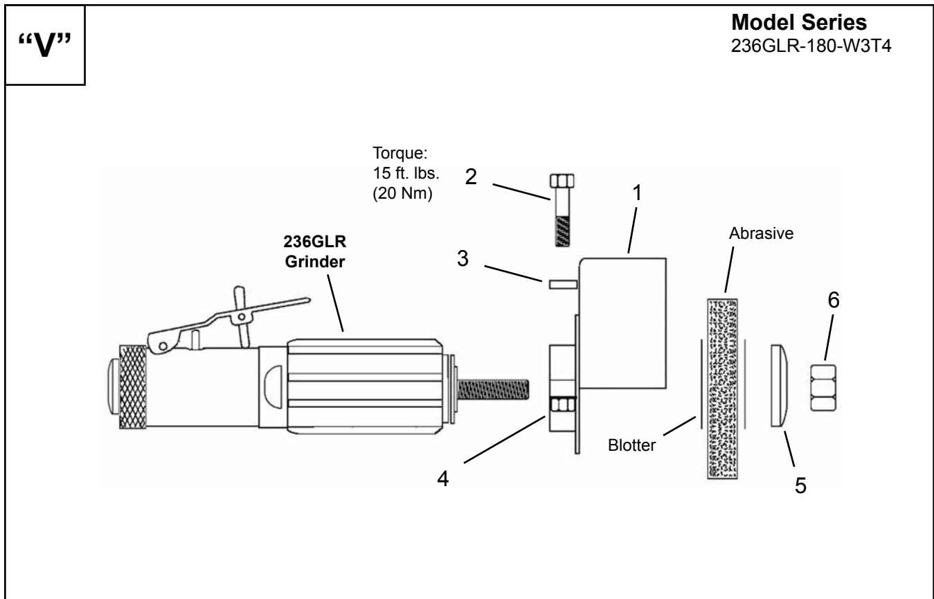
Illustration V: 236G Series Horizontal Grinder Termination W3T4
