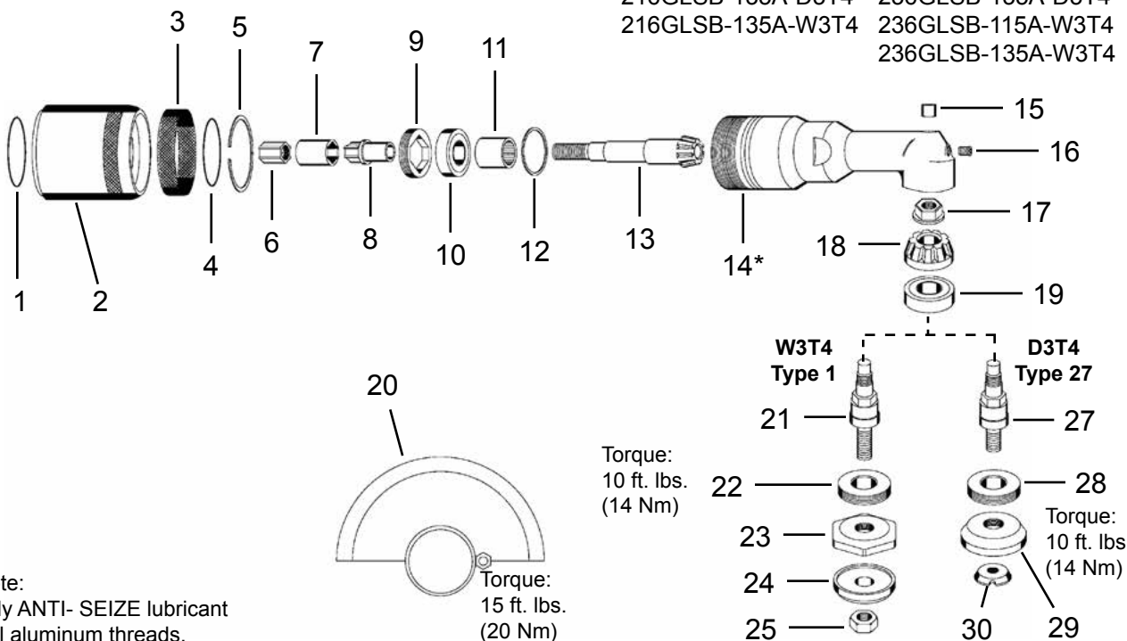
Illustration S: 216G/236G Series Right Angle Front/Side Exhaust Terminations D3T4, W3T4
