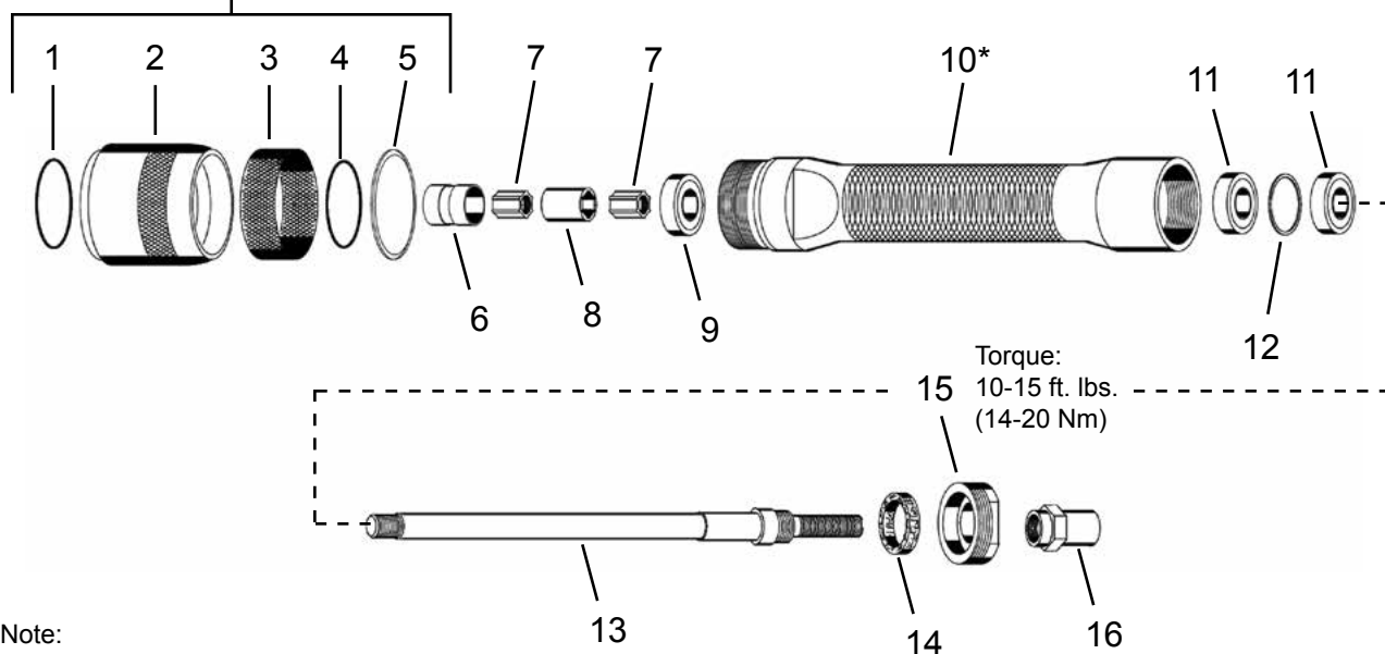
Illustration U: 236G Series Horizontal Extension Grinder Termination P3T
