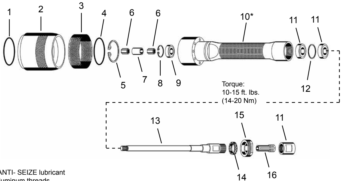
Illustration W: 25G Series Horizontal Extension Grinder Termination C4
