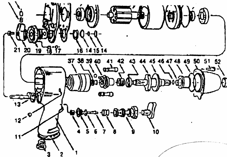
Figure 2 — Replacement Parts Illustration
