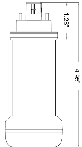
G24d-2 base, 2-pin
