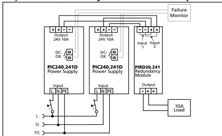
Fig. 23-1 1+1 Redundant wiring with a PIRD20.241 redundancy module
