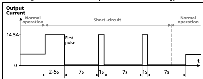
Fig. 6-2 Short-circuit on output, intermittent current, typ.
