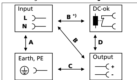
Fig. 18-1 Dielectric strength
