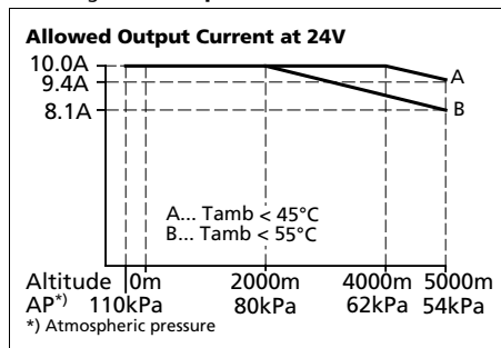
Fig. 16-2 Output current vs. altitude
