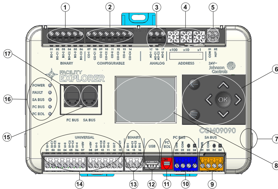
Figure 1: CGM physical features (CGM09090-0H model shown)
