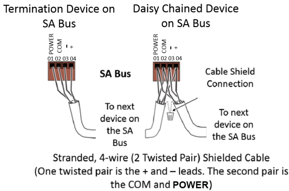
Figure 7: SA Bus Terminal Block Wiring
