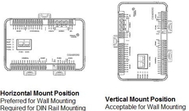
Figure 3: Controller mounting position
