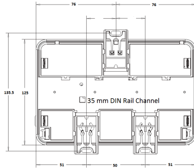
Figure 5: Back of CGE04060 and CGM04060 controller
