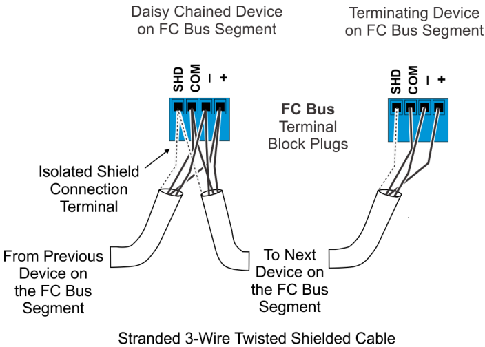
Figure 6: FC Bus terminal block wiring
