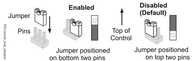
Figure 15: UI Current Loop Jumper Positions
