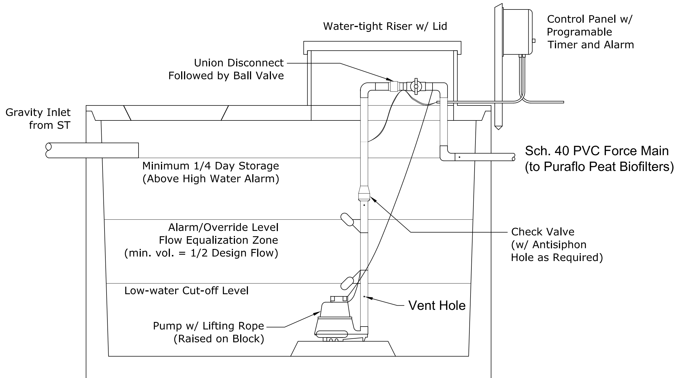
TYPICAL PUMP TANK DETAIL
