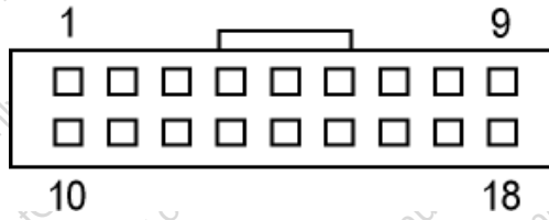
18-pin I/O connector (Looking at the acceptor)
