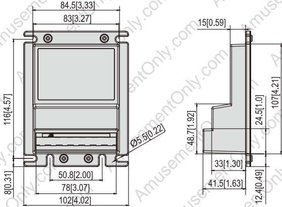
Two Side Bezel (Metal) Part No. 3ZMB-FAC45000
