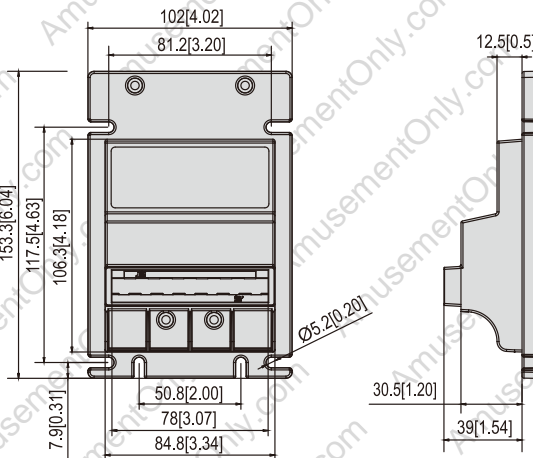
TOB Bezel Part No. 3ZMB-FAC41000
